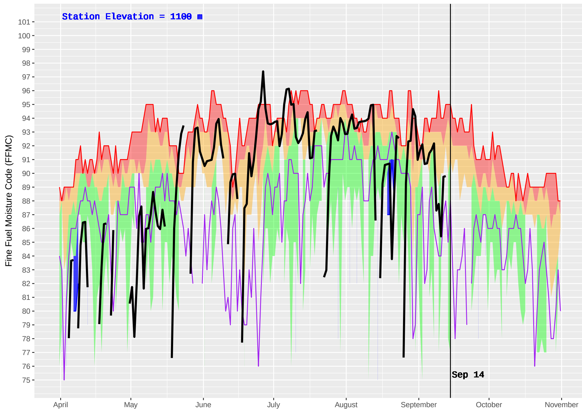
CHURN CREEK (832) : Historical (2003–2016) and Current (2017) Noon Fine Fuel Moisture Code (FFMC)
